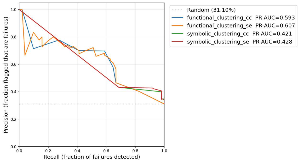
Fig. 6.1. Precision-recall curves for code-specific methods on DeepSeek-Coder-6.7B-Instruct
