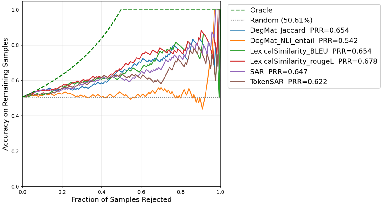
Fig. 6.4. PRR curves for diversity-based methods on DeepSeek-Coder-1.3B-Instruct
