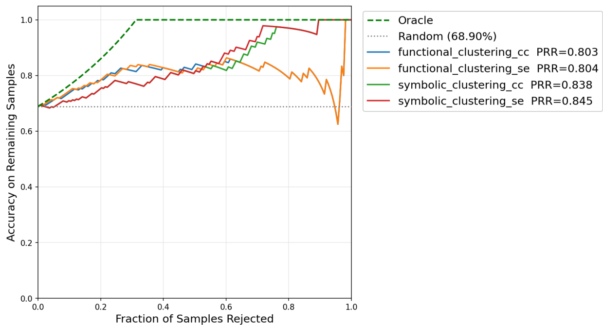
Fig. 6.2. PRR curves for code-specific methods on DeepSeek-Coder-6.7B-Instruct
