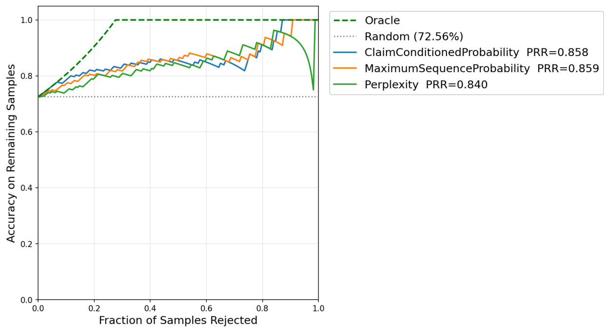
Fig. 6.3. PRR curves for information-theoretic methods on Qwen2.5-Coder-7B-Instruct
